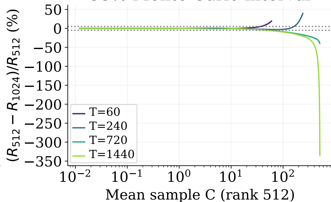
Paired rank difference 95% Monte Carlo interval
